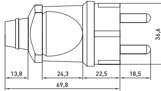
Рис. 2 e.plug.straight.003.16, e.plug.straight.004.16
